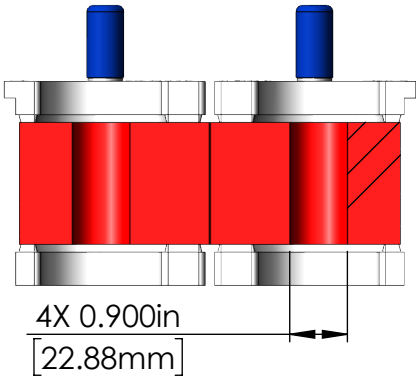
SECTION F-F SCALE 1 : 3
