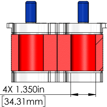
SECTION E-E SCALE 1 : 3
